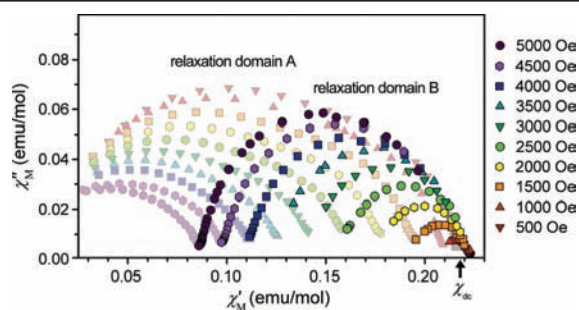
Figure 3. Cole–Cole plots showing the field dependence of multiple relaxation processes occurring in 1 at 1.8 K. Relaxation domains A and B correspond to the ac frequency ranges of 1–1500 and 0.06–1 Hz, respectively. Data in domain A are faded to facilitate visualization. The value of \chi'_{dc} at an applied dc field of 5000 Oe is marked with an arrow to indicate its relation to the low-frequency ac susceptibility data.
